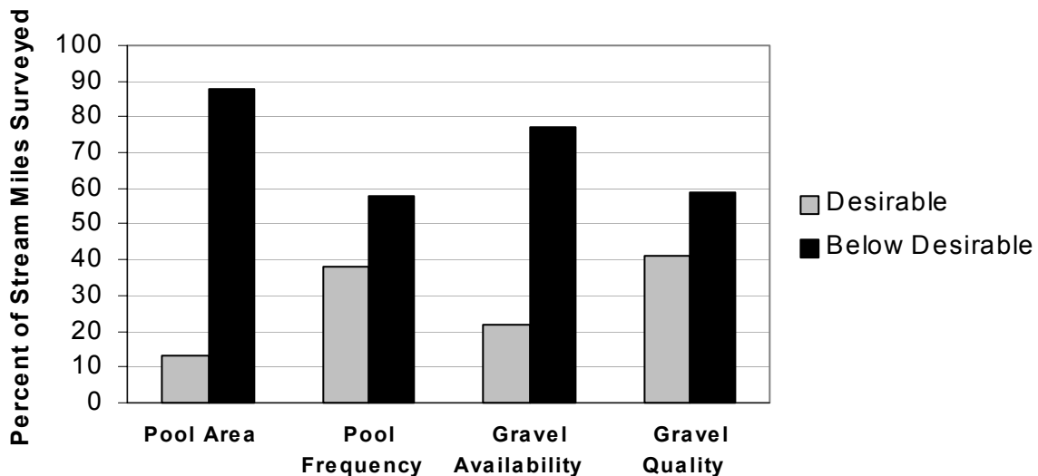
Figure 4-4. Overall habitat ratings for 62 miles of stream surveyed in 1993 and 1994 in the Hood River Watershed. Data source: ODFW, 1995
